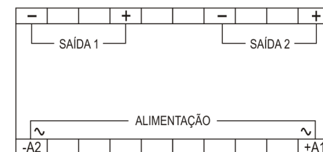
EFCC
