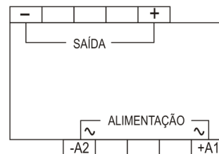
MFCC
